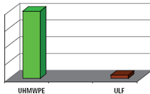
Wear measured as weight loss (gr.) against PET pre-forms
